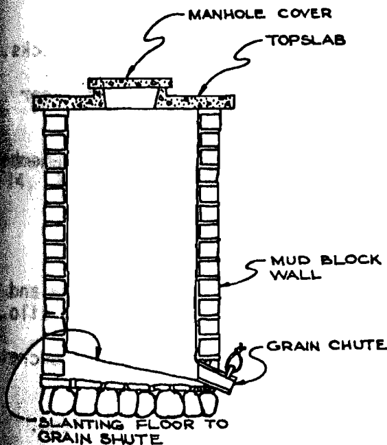
SECTION VIEW THROUGH MUD BLOCK SILO
